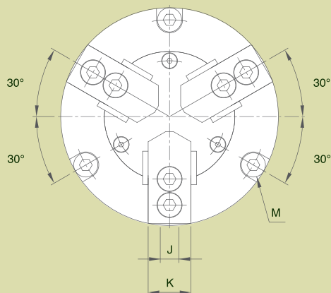
尺寸圖»Dimensions
